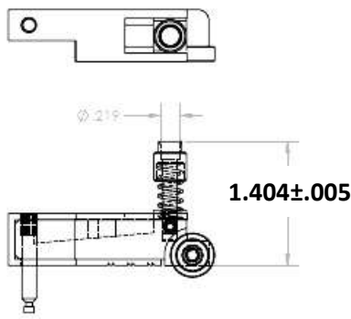
20124, SQ DEAL PRIMER SLIDE LARGE ASSEM
