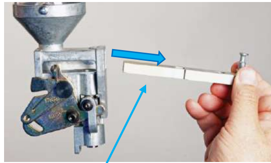
Slide Powder Bar out of the Powder Measure
