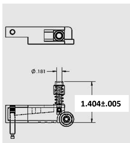
20125, SQ DEAL PRIMER SLIDE SMALL ASSEM
