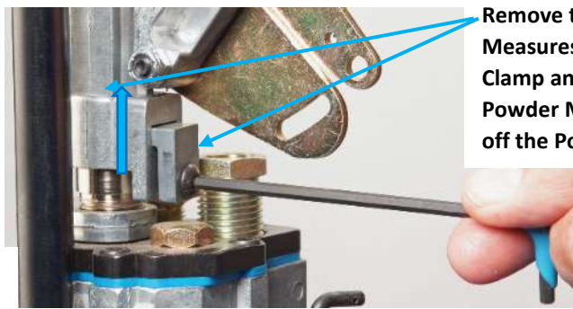
Remove the Powder Measure Failsafe Rod Spring Clip and Failsafe Rod
