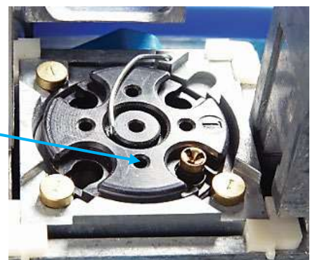
Primer pushed up by Primer Punch ready to be installed if a case was present
